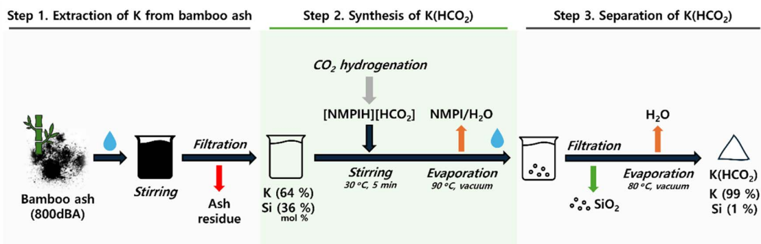
Fig. 4 Production process of K(HCO_2) from 800dBA and 2.
