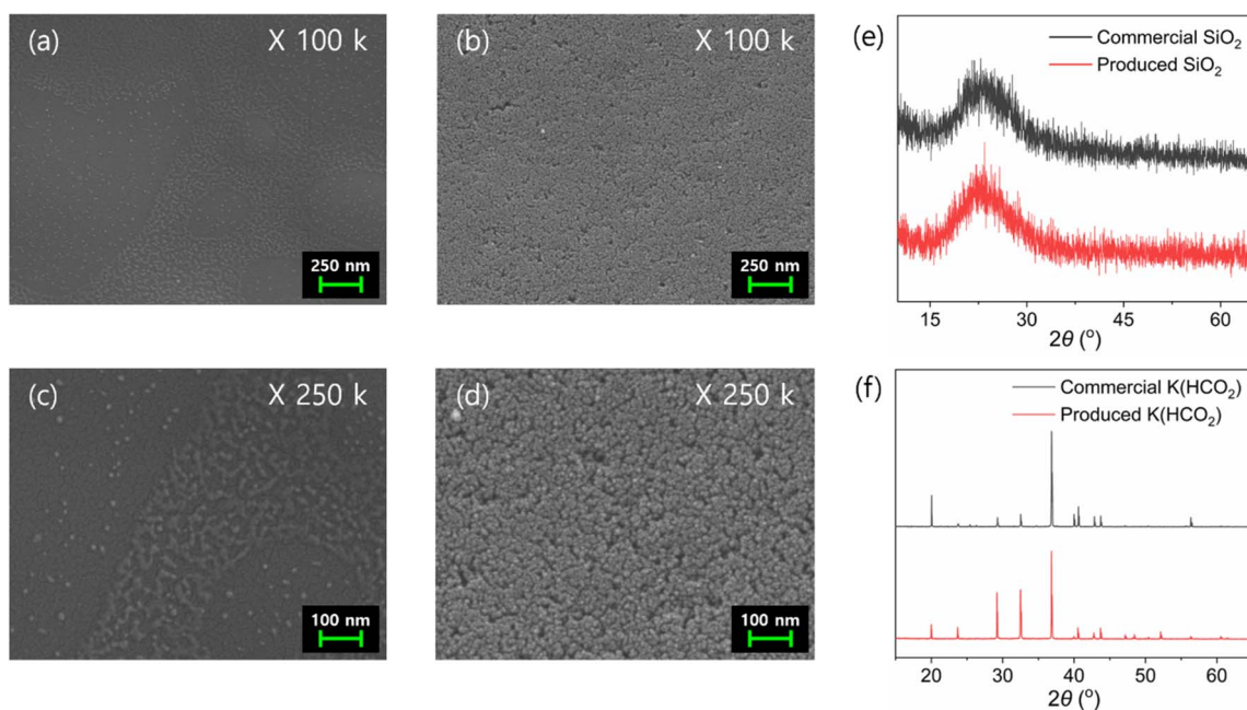
Fig. 5 FE-SEM images of commercial SiO_2 (a and c), SiO_2 filtered during the K(HCO_2) separation step (b and d), XRD spectrums of commercial SiO_2 (black) and SiO_2 filtered during the K(HCO_2) separation step (red) (e), and XRD spectrums of commercial K(HCO_2) (black) and K(HCO_2) produced by using KOH and 2 (red) (f).
